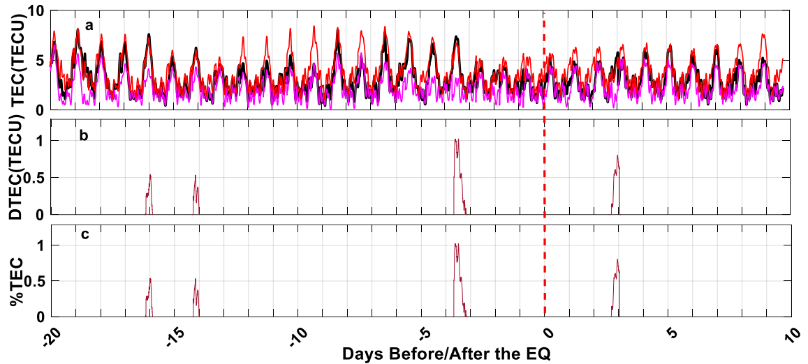
Figure 2.4 (a) Time series of TEC data from Hobs GPS station, (b) DTEC from the same station from Hobs GPS station, and (c) %TEC of the Hobs GPS station Before and after the EQ day. The red dashed line is showing the earthquake day.
