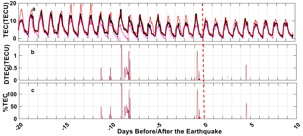
Figure 2.3 (a) Time series of TEC data from COCO GPS station, (b) DTEC from the same station from COCO GPS station, and (c) %TEC of the COCO GPS station before and after the EQ day. The red dashed line is showing the EQ day.
