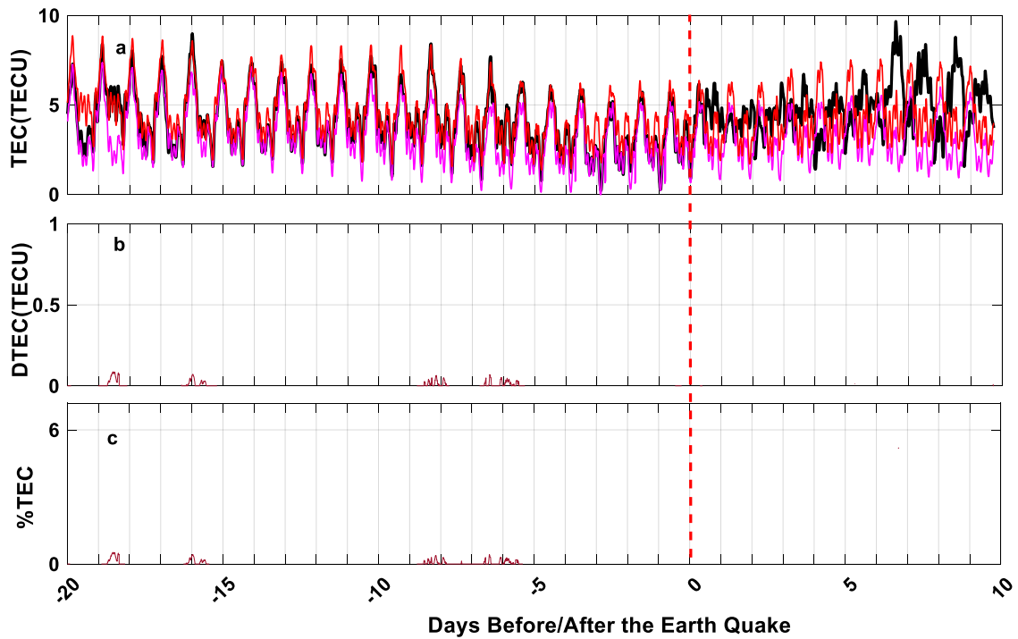
Figure 2.4 (a) Time series of TEC data from Hobs GPS station, (b) DTEC from the same station from Hobs GPS station, and (c) %TEC of the Hobs GPS station Before and after the EQ day. The red dashed line is showing the earthquake day.
