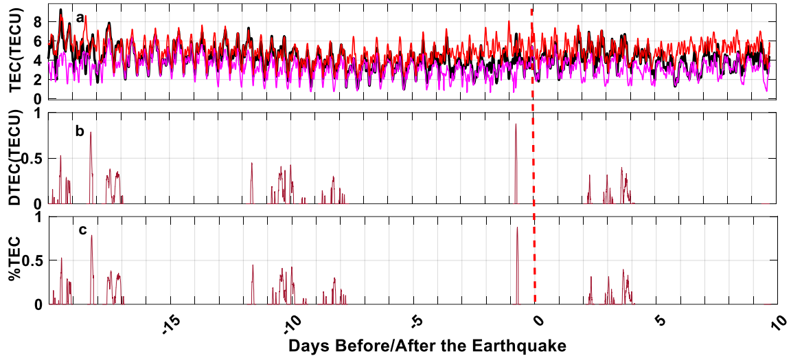
Figure 2.6 (a) Time series of TEC data from AUCK GPS station, (b) DTEC from the same station from AUCK GPS station, and (c) %TEC of the AUCK GPS station before and after the EQ day. The red dashed line is showing the EQ day.
