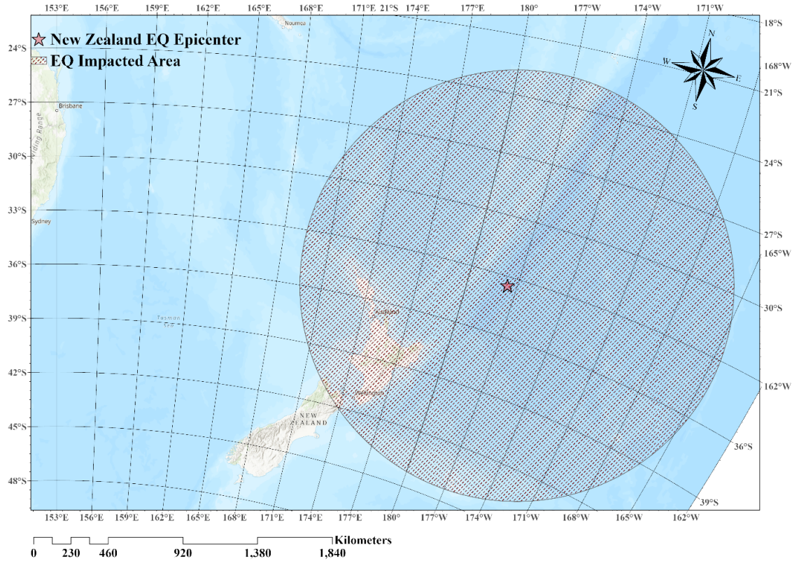
Fig. 2. 1 Location of the EQ epicenter. Red star shows the coordinates of epicenter
