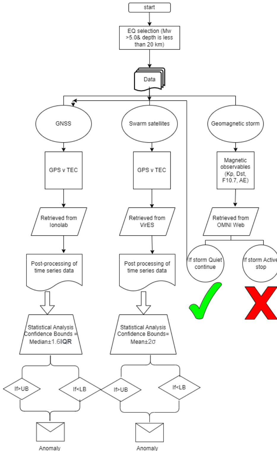
Figure 2.3 Flow chart of the methodology executed in this study for finding abnormal variation in the ionosphere associated with the EQ of Magnitude 7.4
