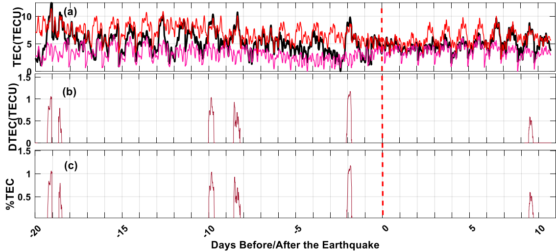
Figure 2.2 (a) Time series of TEC data from TIDB GPS station, (b) DTEC from the same station from TIDB GPS station, and (c) %TEC of the TIDB GPS station before and after the EQ Day. The red dashed line is showing the EQ day. The bold black line represents TEC. Red and Pink line represent the confidence bounds.
